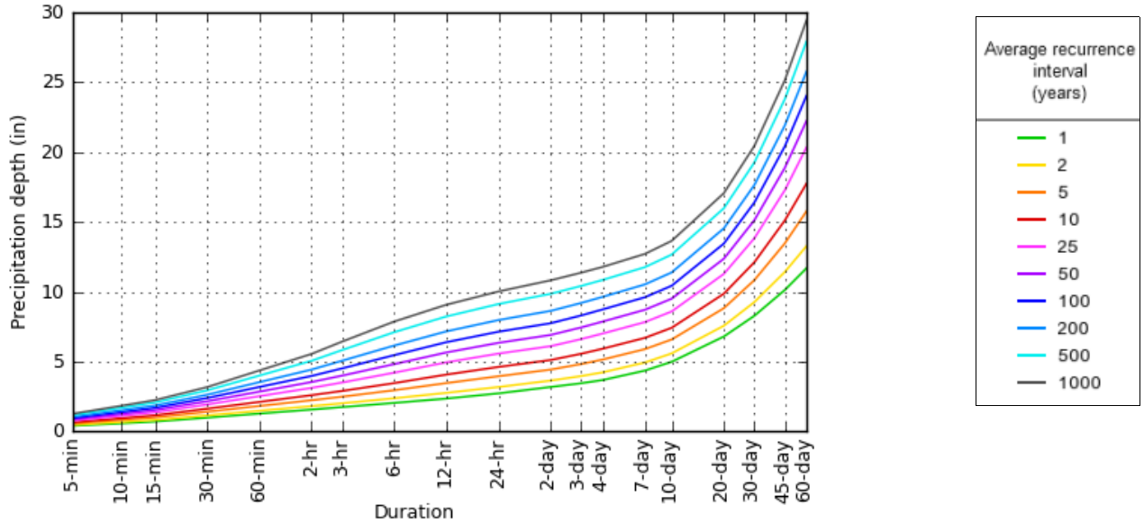
PDS-based depth-duration-frequency (DDF) curves Latitude: 40.4007°, Longitude: -91.3865°
